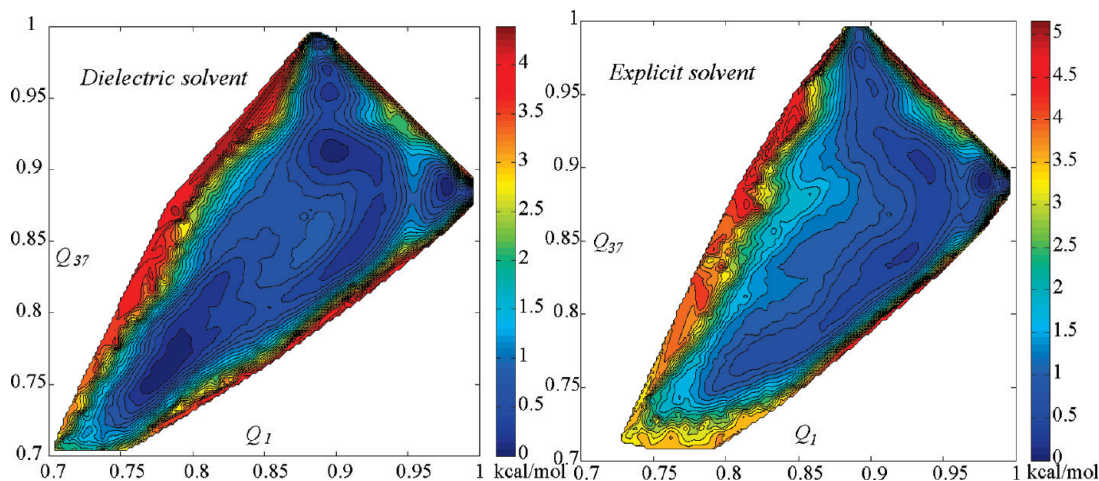
Figure 9. (left) FES computed for the dielectric solvent model on the left. (Right) Explicit solvent FES. The lower basin is absent in the explicit solvent FES. On the other hand, a number of barriers have disappeared in the DSM FES. The vicinities of the reference points 1 and 37 are very similar between explicit and DSM FESs.
